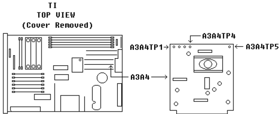
Figure 18. A3A4 Card.
