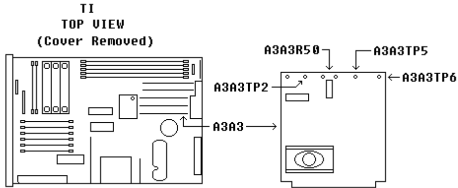
Figure 17. A3A3 card.
